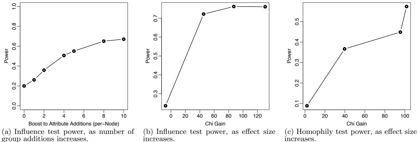
Figure 2: Power analysis of influence and homophily randomization tests.
