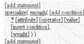
Figure 10. Procedure specializeIfEnough.
